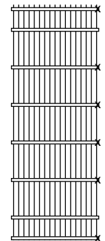
H 2430 mm M 50/200/400 mm P Ø 60 mm
