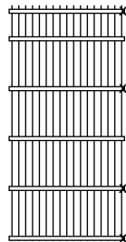
H 1830 mm M 50/200/400 mm P Ø 48 mm
