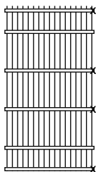
H 1630 mm M 50/200/400 mm P Ø 48 mm
