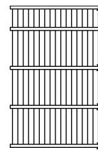
H 1430 mm M 50/200/400 mm P Ø 48 mm
